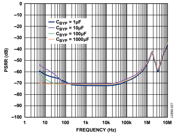
Figure 27. Power Supply Rejection Ratio (PSRR) vs. Frequency at Various C_{BYF} Values, V_{OUT} = 3.3\text{ V} , V_{IN} = 4.0\text{ V} , 2 A Load
