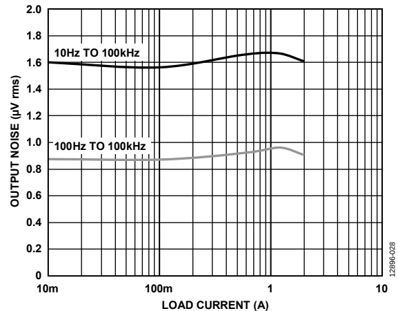
Figure 28. RMS Output Noise vs. Load Current
