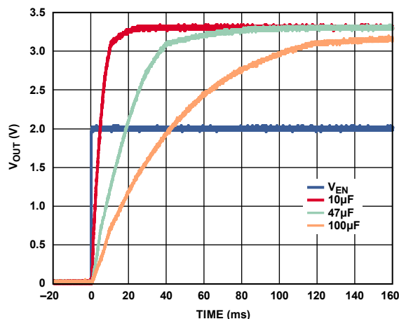
Figure 53. Typical Start-Up Behavior with C_{BYP} = 10 \mu\text{F} to 100 \mu\text{F}
